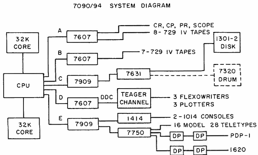
Figure 1.1 7090/94 System Diagram
