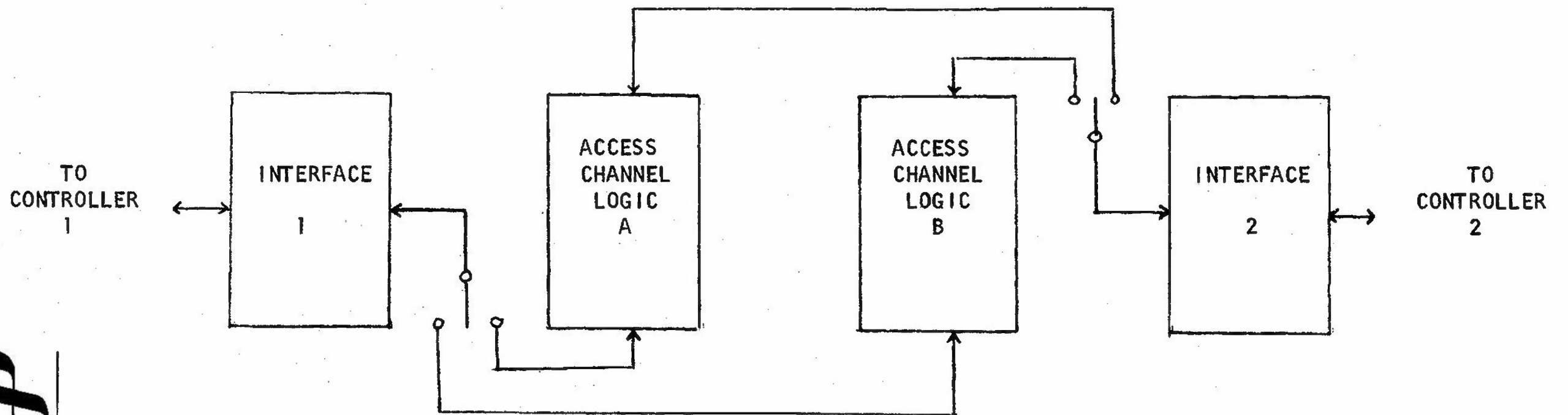
FIGURE 1B. DUAL-SWITCH CONFIGURATION
