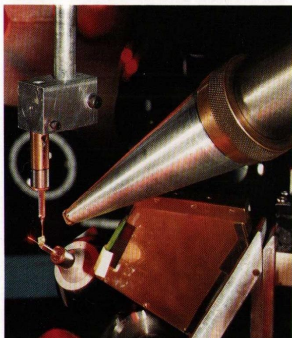
Dense plasmas are formed when two lasers are focused on to a thin foil of plastic coated aluminium. The spacing between the ions in these plasmas can then be measured by using laser-produced X-rays.
