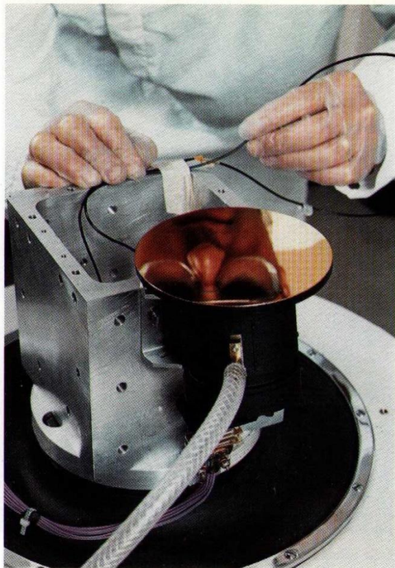
This highly polished mirror is part of the ATSR system to measure the temperature of the sea surface from 500 miles up in space. The mirror will rotate six times a second throughout the three year mission.
