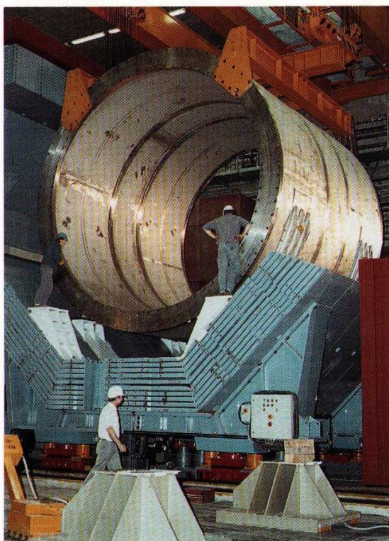
The huge magnet built at RAL for the H1 particle physics experiment in Hamburg is one of the largest in the world.
