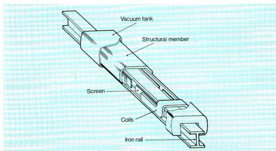
Fig 16 A possible magnetic levitation system for high speed transport.
