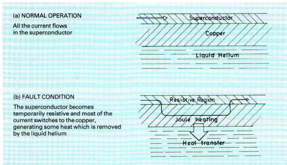
Fig 3 The principles of cryostabilization.
