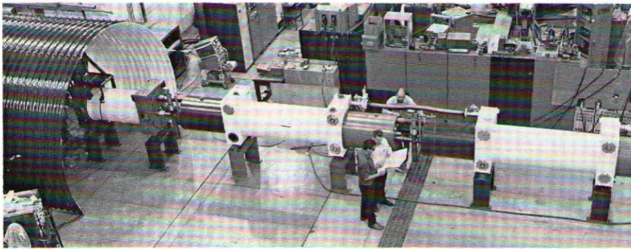
Fig 11 Testing a prototype section of the superconducting accelerator ISABELLE. (Photograph courtesy of the Brookhaven National Laboratory, USA.)
