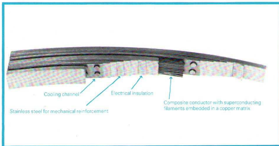
Fig 4 A typical cryostabilized conductor.
