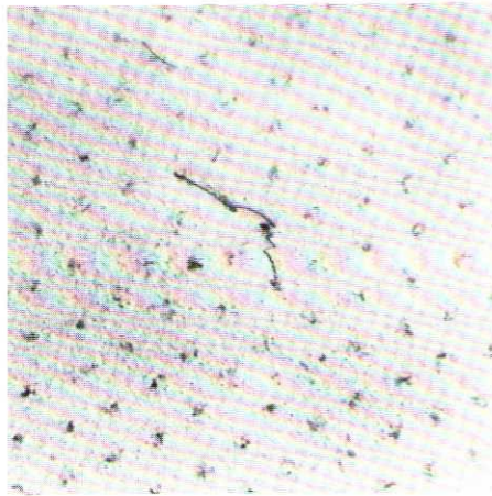
Fig 1 Discrete flux lines in superconducting niobium. Each line consists of a normal core surrounded by a vortex of supercurrent. The lines tend to form a regular array, but this is distorted by the lattice dislocation in the niobium crystal visible as a jagged line in the centre of the picture. (Photograph courtesy of C P Herring.)
