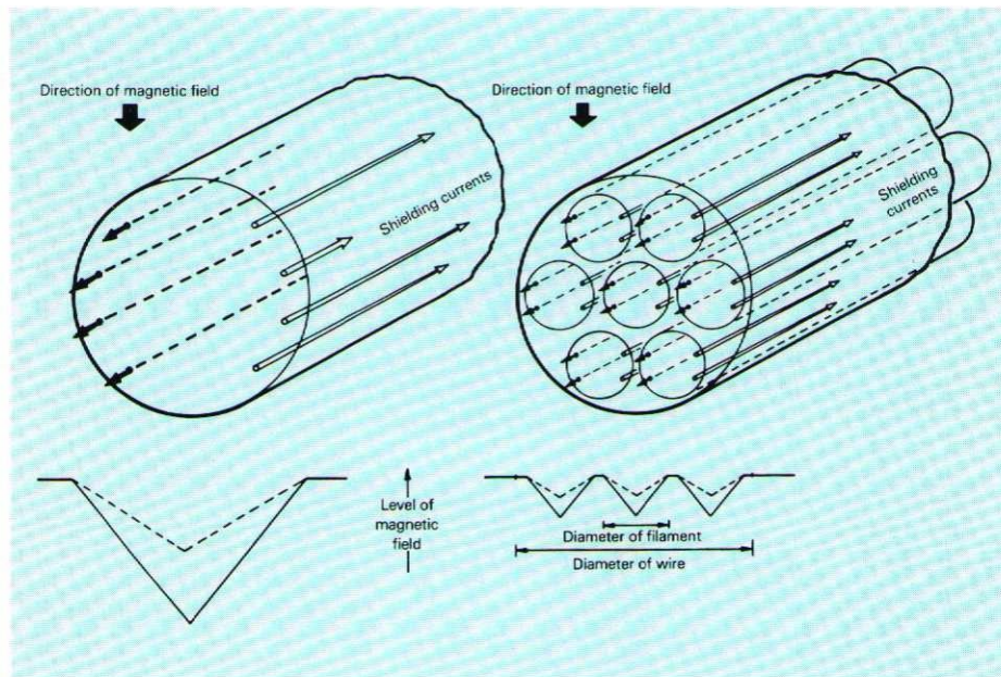
Fig 6 Screening currents induced in a superconducting wire by a magnetic field. These currents are prone to an instability known as 'flux jumping'. The extent of the currents, the amplitude of the screened field and the likelihood of flux jumping may all be reduced by fine subdivision, as shown in the right-hand diagram.
