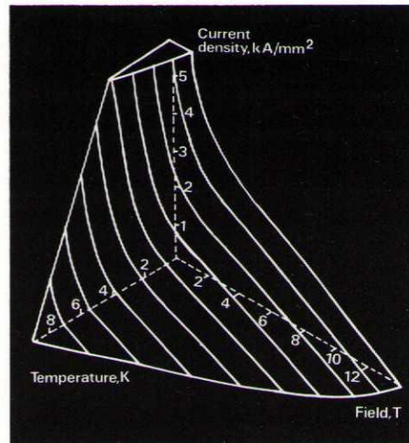
Fig 2 The critical surface for niobium titanium alloy. Superconductivity prevails below the surface, and normal resistivity above the surface.
