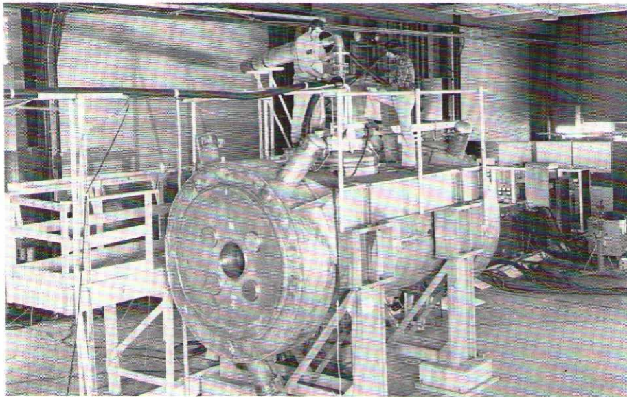
Fig 13 A large superconducting dipole magnet for experiments in magnetohydrodynamic power generation. (Photograph courtesy of the Argonne National Laboratory, USA.)
