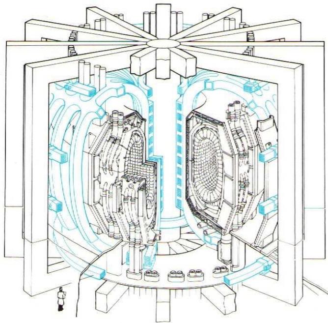
Fig 12 Conceptual design for a 2,500 megawatt power generating Tokamak fusion reactor. (Design courtesy of the Culham Laboratory.)
