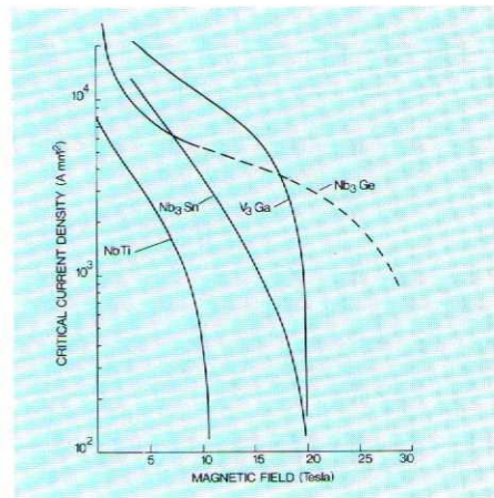
Fig 9 The critical current densities of some high field superconducting materials.
