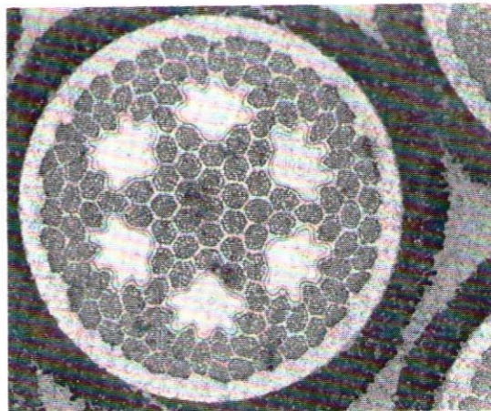
Fig 10 Cross-sectional view of a filamentary niobium tin magnet showing the 0.5 mm diameter wires insulated by glass-fibre and encapsulated in epoxy resin. Each wire contains 4,477 filaments of niobium tin of about 3 micron diameter in a bronze matrix with 6 large filaments of pure copper. (Photograph courtesy of AERE Harwell.)
