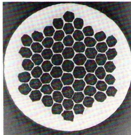
Fig 7 Cross-sectional view of a 61-filament superconducting composite wire. The overall wire diameter is about 0.5 mm and the diameter of each filament is about 40 micron. The filament material is niobium titanium and the matrix material is copper. (Photograph courtesy of Imperial Metal Industries Limited.)
