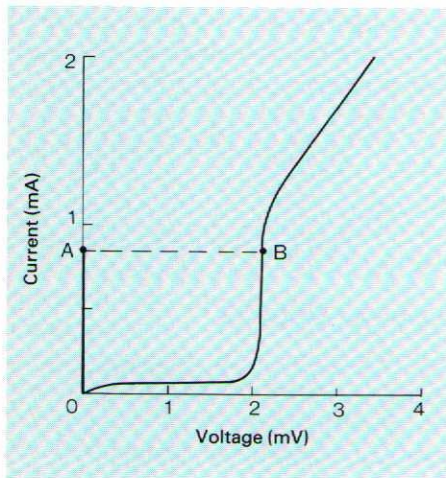
Fig 17 Typical characteristics of a Josephson junction of tin/tin oxide/tin at 1.8 K. Branch OA is attributed to supercurrent tunnelling and OB is tunnelling by normal electrons.
